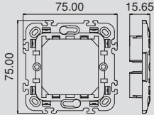
Metal Mounting Frame 2M
