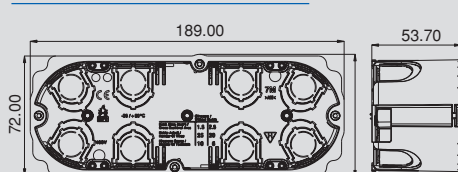
Hollow Wall Box 7M
