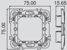
Mounting Frame 2M
