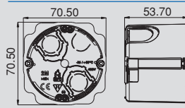
Hollow Wall Box 2M
