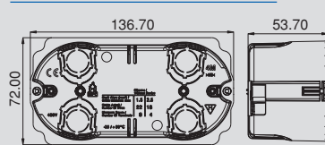
Hollow Wall Box 4M
