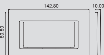
Optima 4M Frame
