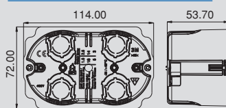
Hollow Wall Box 3M
